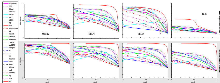
Fig. 6. Accuracy of saliency detection models over least and most consistent images
