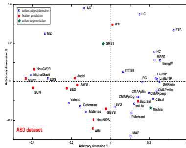
Fig. 9. Measuring model similarities
