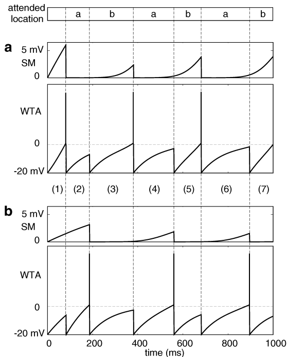
Figure 4: Dynamical evolution of the potential of some simulated neurons in the saliency map (SM) and in the winner-take-all (WTA) networks. The input contains one salient location (a), and another input of half the saliency (b); the potentials of the corresponding neurons in the SM and WTA are shown as a function of time. During period (1), the potential of both SM neurons (a) and (b) increases as a result of the input. The potential in the WTA neurons, which receive inputs from the corresponding SM neurons but have much faster time constants, increases faster. The WTA neurons evolve independently of each other as long as they are not firing. At about 80ms, WTA neuron (a) reaches threshold and fires. A cascade of events follows: First, the focus of attention is shifted to (a); second, both WTA neurons are reset; third, inhibition-of-return (IOR) is triggered, and inhibits SM neuron (a) with a strength proportional to that neuron's potential (i.e., more salient locations receive more IOR, so that all attended locations will recover from IOR in approximately the same time). In period (2), the potential of WTA neuron (a) rises at a much slower rate, because SM neuron (a) is strongly inhibited by IOR. WTA neuron (b) hence reaches threshold first. (3)-(7): In this example with only two active locations, the system alternatively attends to (a) and (b). Note how the IOR decays over time, allowing for each location to be attended several times. Also note how the amount of IOR is proportional to the SM potential when IOR is triggered (e.g., SM neuron (a) receives more IOR at the end of period (1) than at the end of period (3)). Finally, note how the SM neurons do not have an opportunity to reach threshold (at 20 mV) and to fire (their threshold is ignored in the model). Since our input images are noisy, we did not explicitly incorporate noise into the neurons' dynamics.
