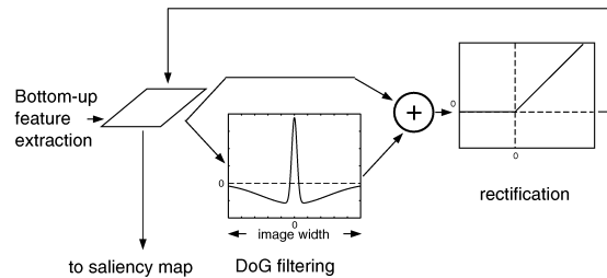
Figure 2: Illustration of the spatial competition for salience implemented within each of the 42 feature maps. Each map receives input from the linear filtering and center-surround stages. At each step of the process, the convolution of the map by a large Difference-of-Gaussians (DoG) kernel is added to the current contents of the map. This additional input coarsely models short-range excitatory processes and long-range inhibitory interactions between neighboring visual locations. The map is half-wave rectified, such that negative values are eliminated, hence making the iterative process non-linear. Ten iterations of the process are carried out before the output of each feature map is used in building the saliency map.
